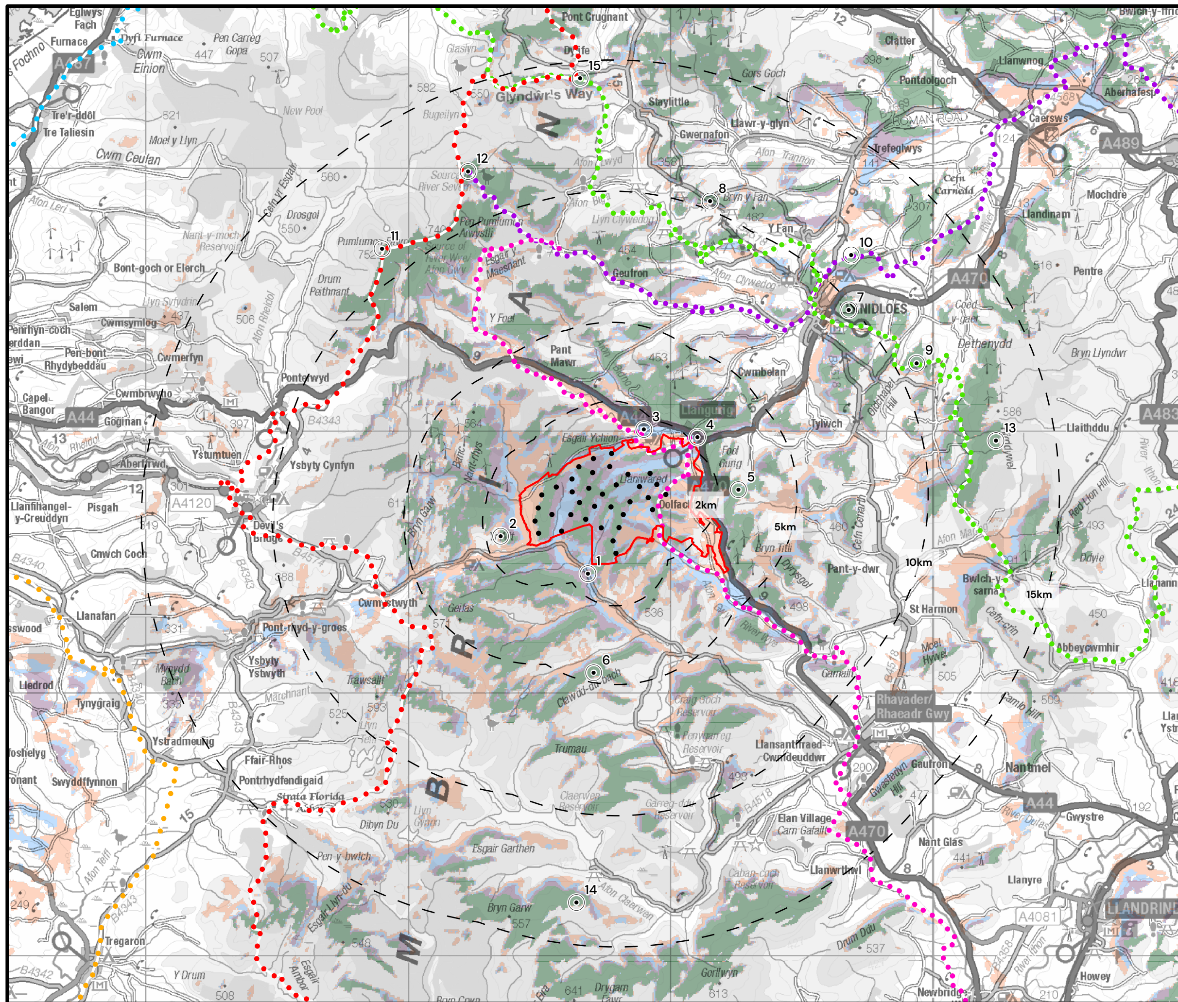
FIGURE 5.3 TURBINE HUB HEIGHT (149M) ZONE OF THEORETICAL VISIBILITY (ZTV)
